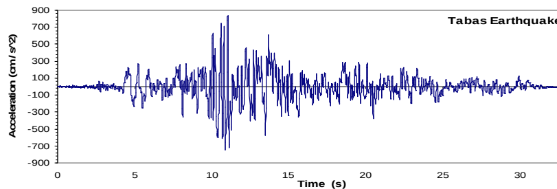
Fig. 1-b Mapping Tabas earthquake acceleration
