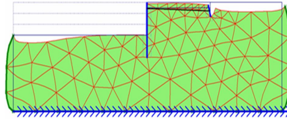
Fig. 4: the sheet pile system deformation mesh for 1m anchor depth
