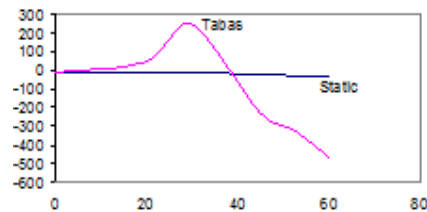
Fig. 6: studying the effect of anchors angles on the horizontal displacement of top sheet pile
