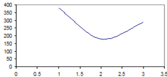
Fig. 5: studying the effect of anchors depth on the maximum horizontal displacement of sheet pile
