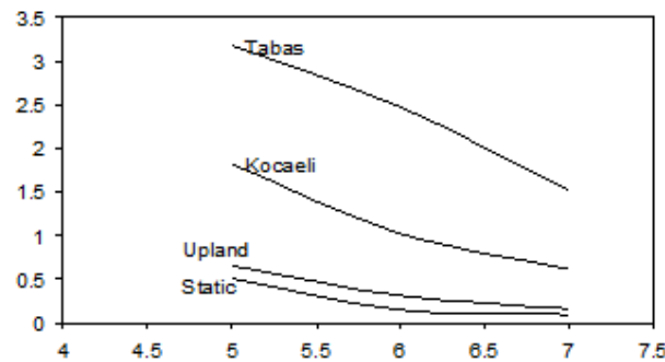
Fig. 2: the horizontal displacement top non-anchored sheet pile for the buried depth
