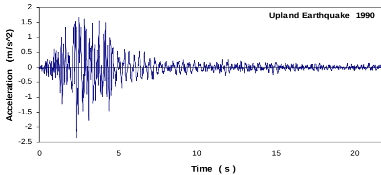
Fig. 1-c. Mapping Upland (1990) earthquake acceleration
