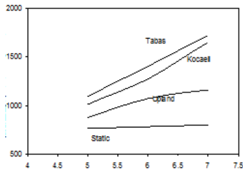
Fig. 3: maximum bending anchor of non-anchored sheet pile for the buried depth
